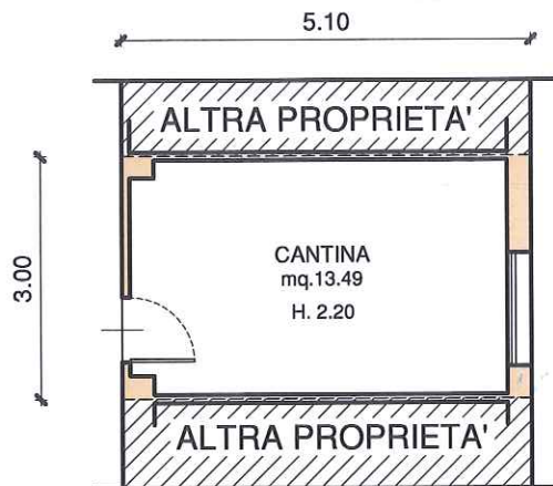
PIANO SEMINTERRATO - 1:100
